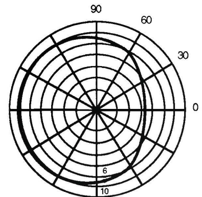
Typical Horizontal Pattern with Reflector
