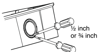
Figure 17 Knockout and V500/V700 Removal for Surface Mount Back Box
