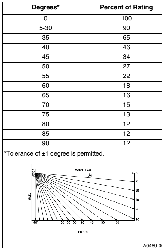
Figure 4 Vertical Dispersion– Wall to Floor
