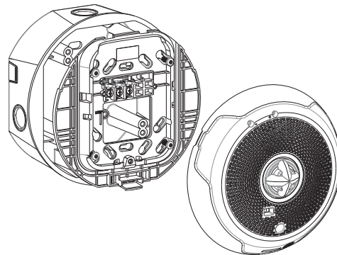
Figure 13 Surface Mounting a Ceiling Device (SBBCRL/SBBCWL)
