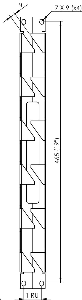
VISTA FRONTAL
