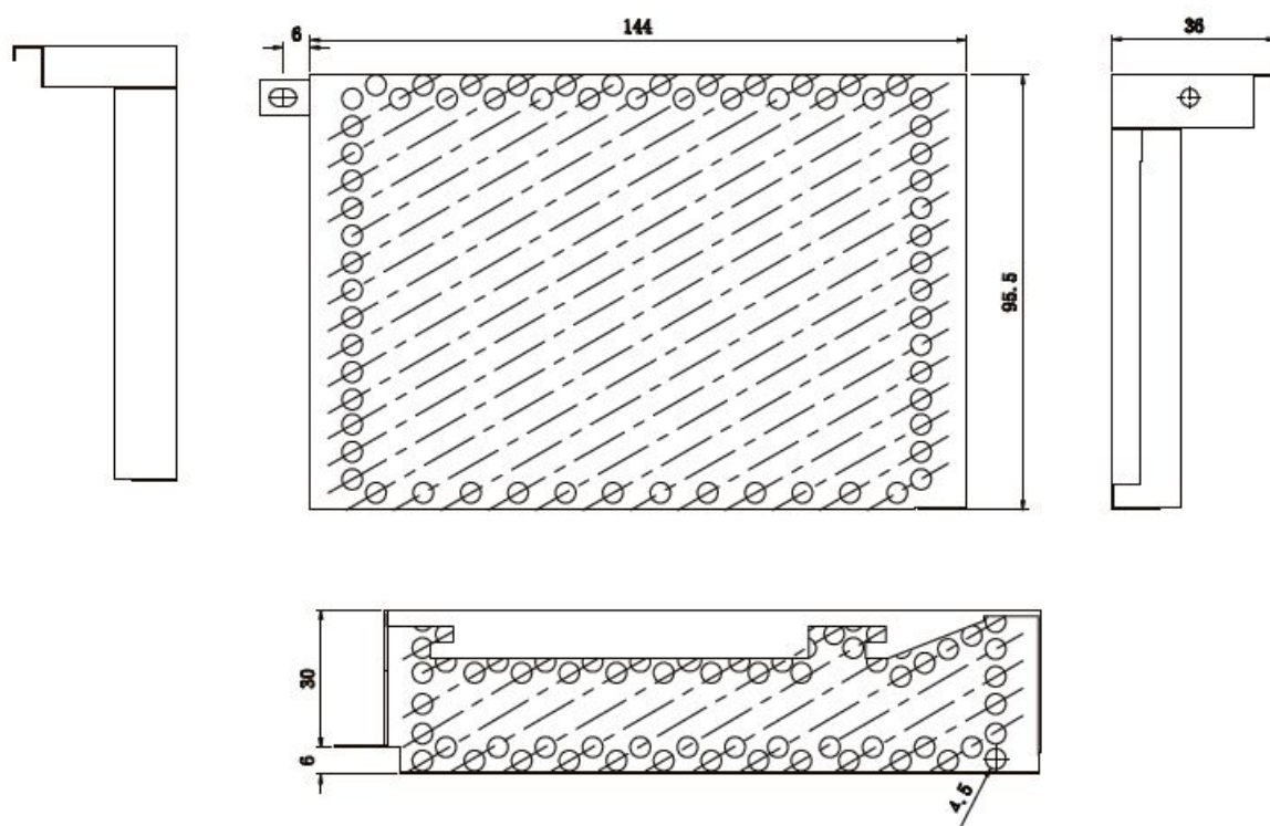
Upper Cover
