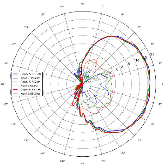
CH 4 Horizontal Polarization, Azimuth
