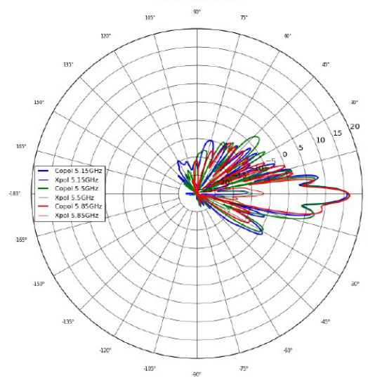
CH 4 Horizontal Polarization, Elevation
