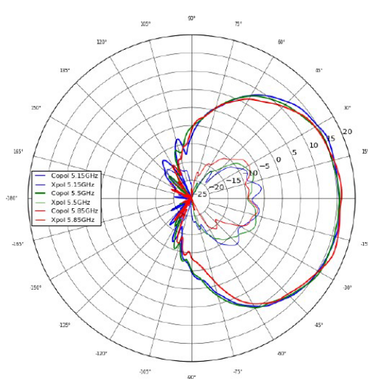
CH 5 Vertical Polarization, Azimuth
