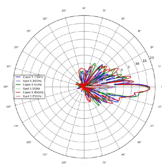
CH 1 Vertical Polarization, Elevation
