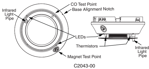
FIGURE 4. CLEANING THE FIRE/CO DETECTOR
