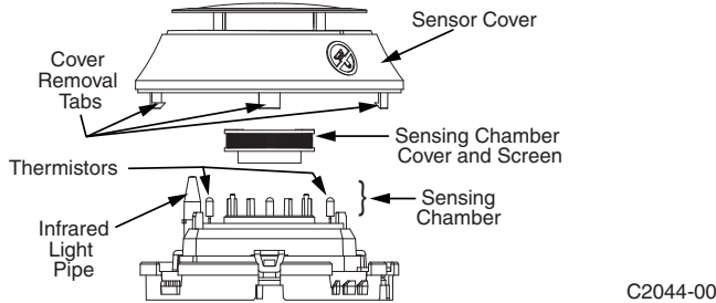
FIGURE 4. CLEANING THE FIRE/CO DETECTOR
