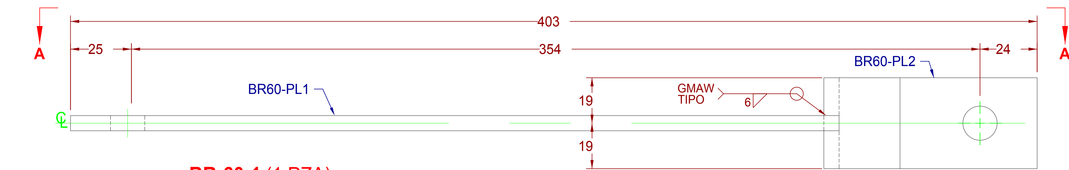
BR-60-1 (1 PZA) PLACA 1/4" X 1 1/2"
