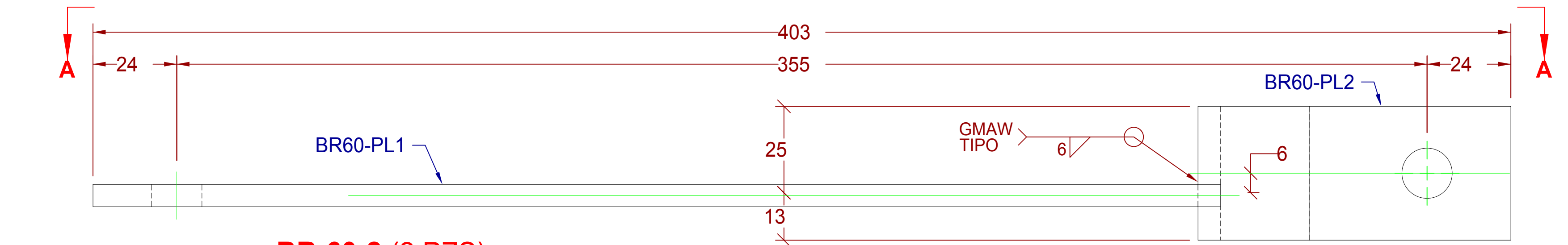
BR-60-2 (2 PZS) PLACA 1/4" X 1 1/2"
