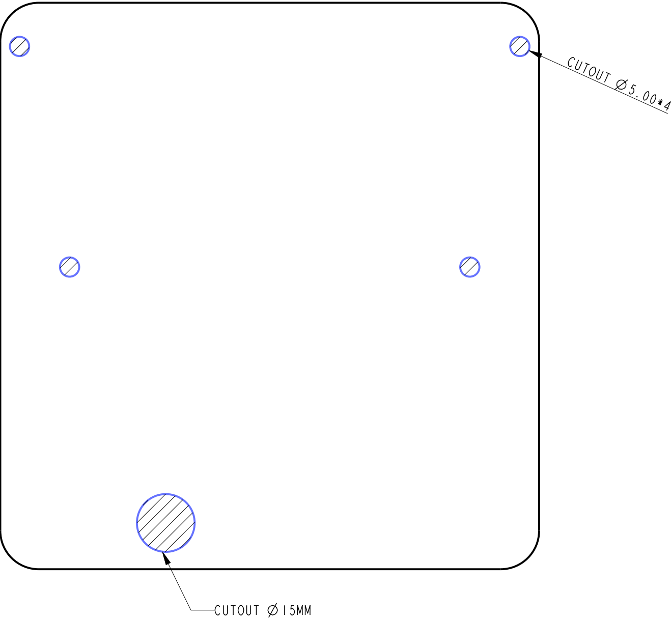
E400 Mounting Template
